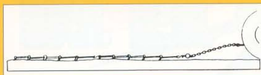
Aggressive action: Tines stand up at 75° angle.
